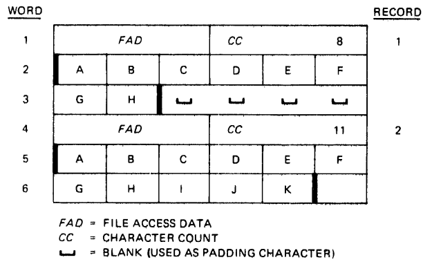
Figure 8-12 Variable-Length SIXBIT
