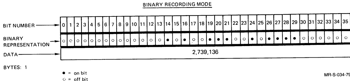
Figure 8-5 Binary Recording Mode
