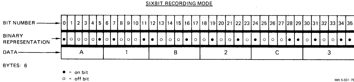
Figure 8-2 SIXBIT Recording Mode
