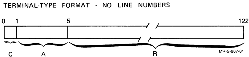
Figure 1-3(a): Terminal-Type Format without Line Numbers
