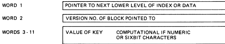
Figure 8-27 ISAM Index File Structure
