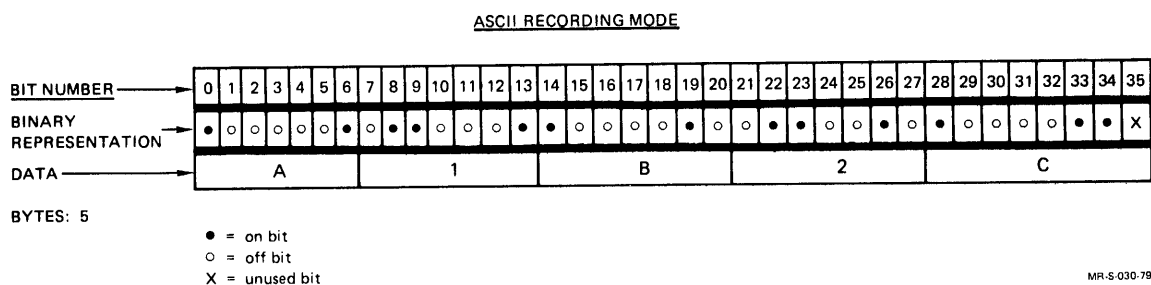
Figure 8-1 ASCII Recording Mode
