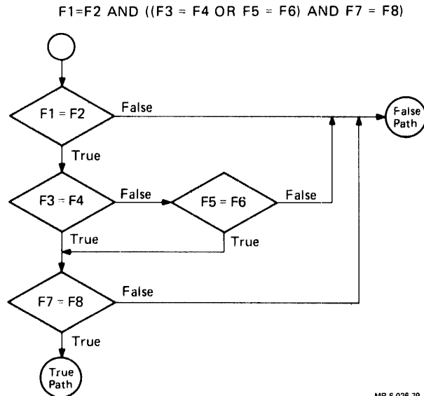
Figure 5-2 Order of Evaluation of a Compound-conditional Expression
