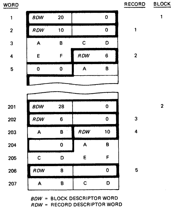
Figure 8-19 Blocked Variable-Length EBCDIC
