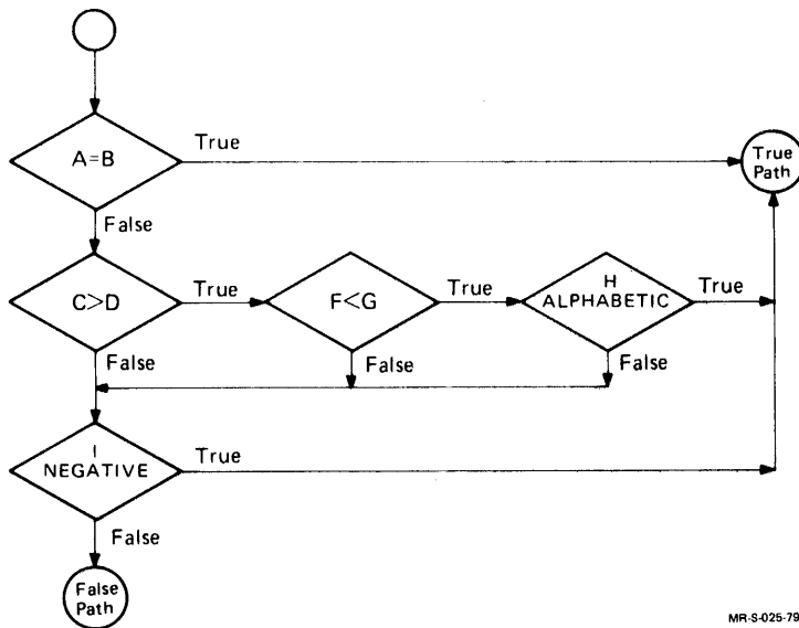
Figure 5-1 Order of Evaluation of a Conditional Expression
