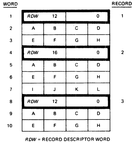
Figure 8-16 Variable-Length EBCDIC
