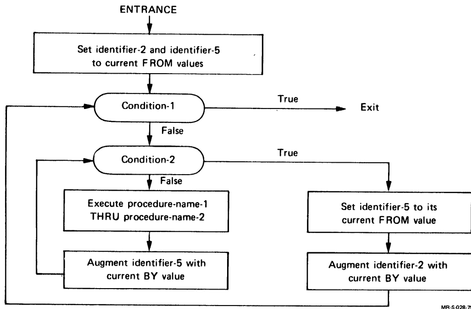
Figure 5-3 PERFORM Cycle Logic - Two Variables
