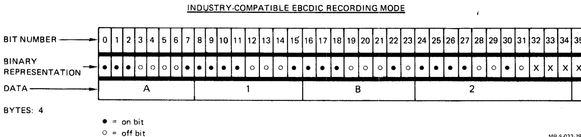
Figure 8-4 EBCDIC Recording Mode - Industry-Compatible
